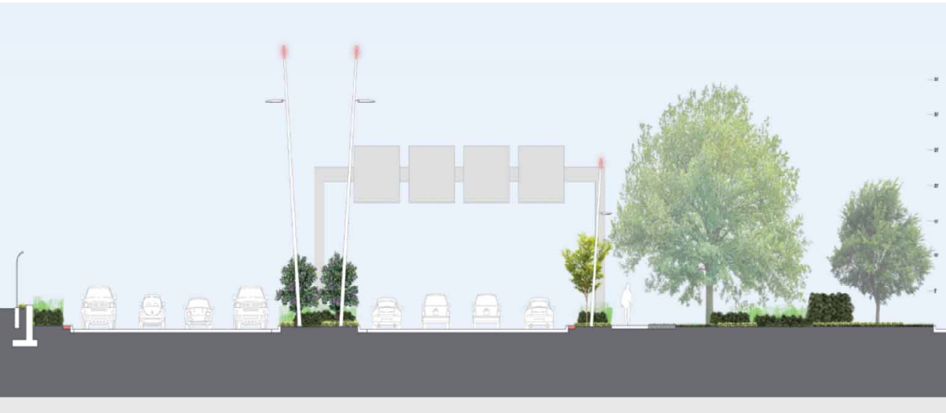
Herb Kelleher Way Streetscape Section
