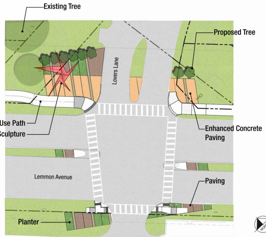
LOVERS LANE SECONDARY GATEWAY ENLARGEMENT SCALE: 1" = 20'
