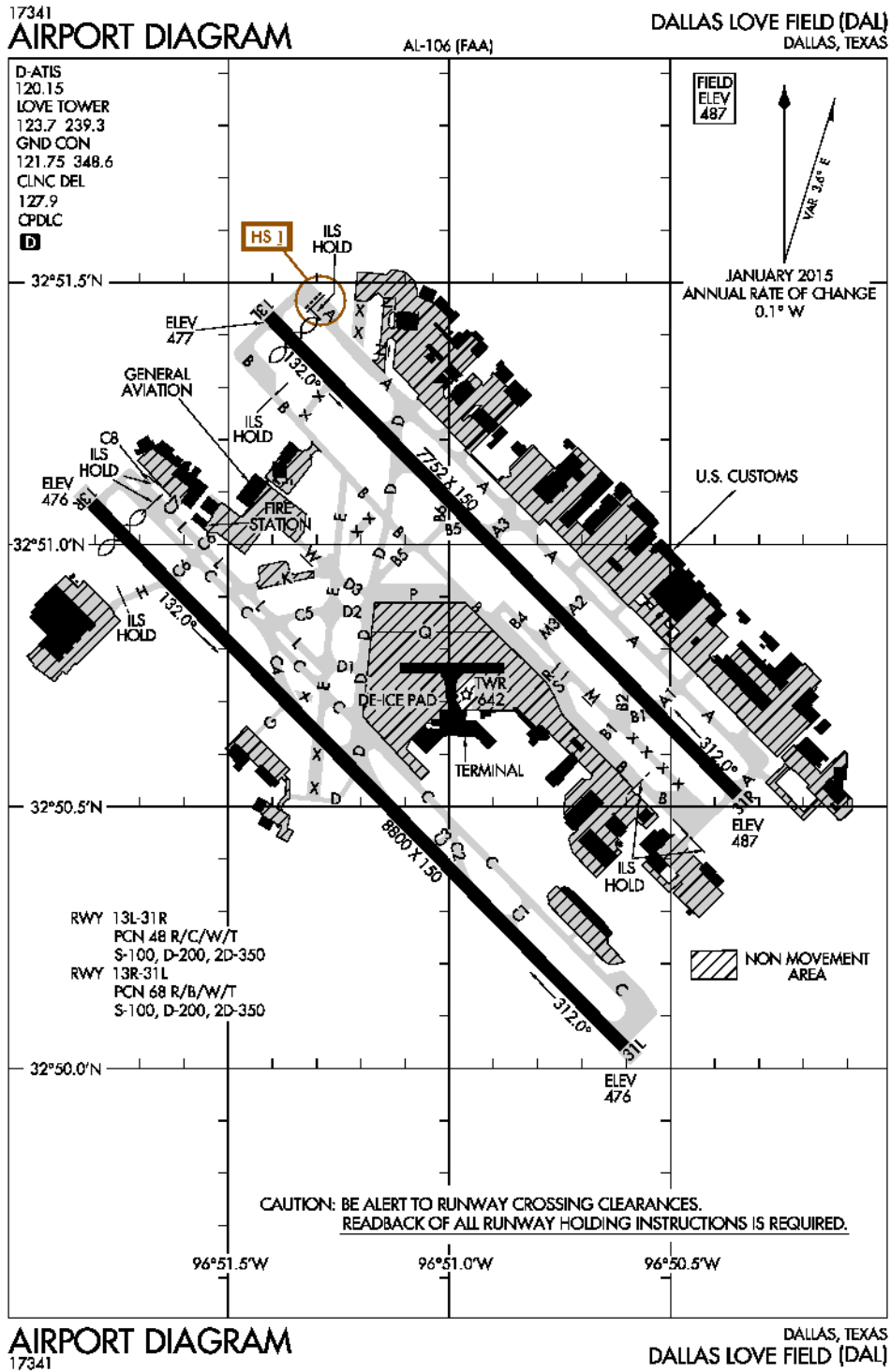
Figure 12. Dallas Love Field Airport Diagram
